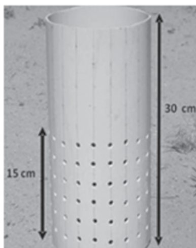
Fig. 7.1: Field water tube
