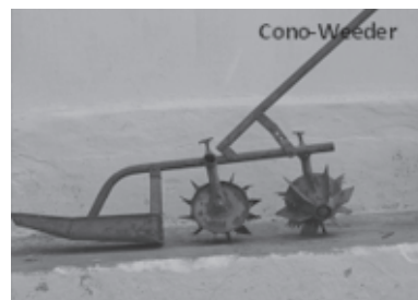
Fig. 5.8: Inter-culture implements
