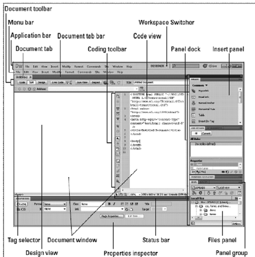
Fig 5.2: Adobe Dreamweaver's Environment
