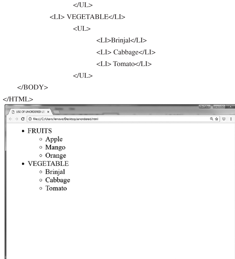
Fig. 2.9: Displaying Unordered Lists in browser
