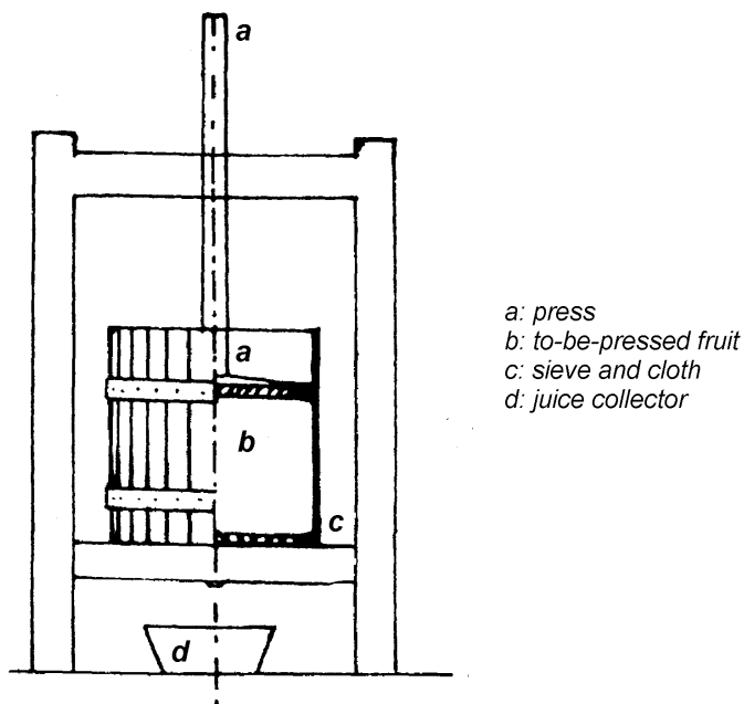
Figure 11: Fruit press
